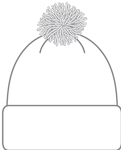
6 Seam Watch Cap (with or without pom)
